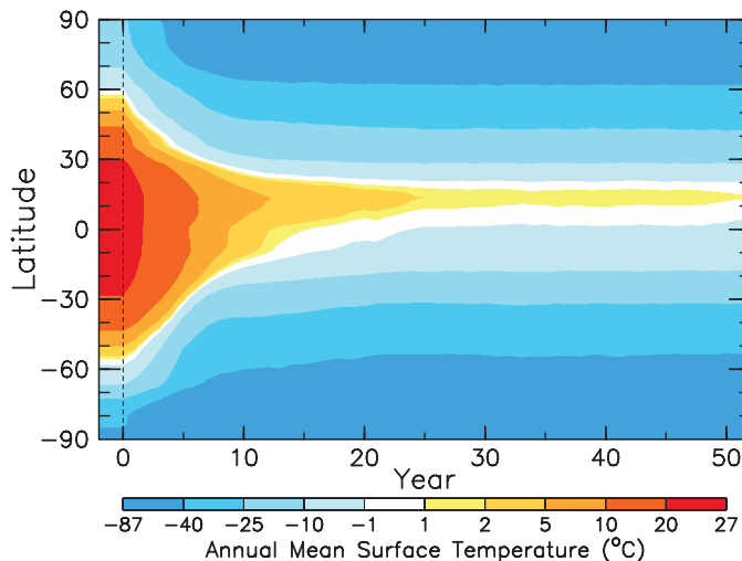
Fig. 3. Zonally averaged annual mean surface temperature change after the zeroing out of noncondensing GHGs.
